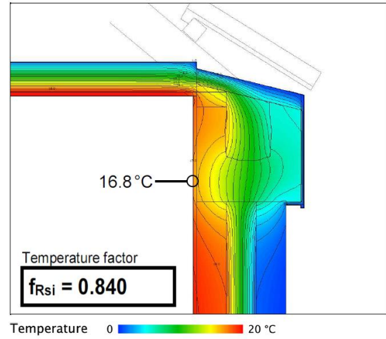
Solid Concrete Gutter Detail – 10mm & 20mm Spaceloft® applied externally
