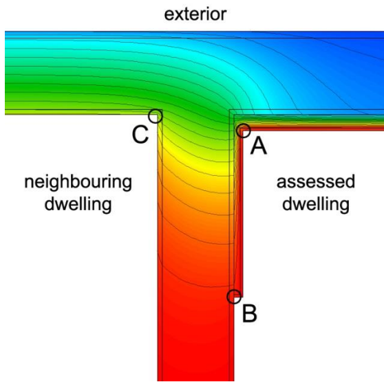
Thermal Bridge at treated & non treated properties
