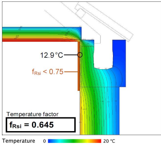
Solid Concrete Gutter Detail – Before
